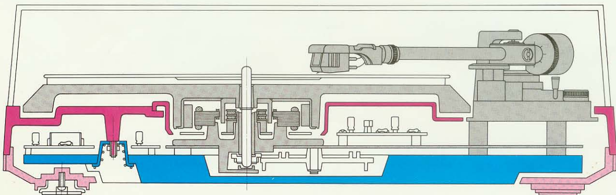
Cross Section of SL-1300MK2
